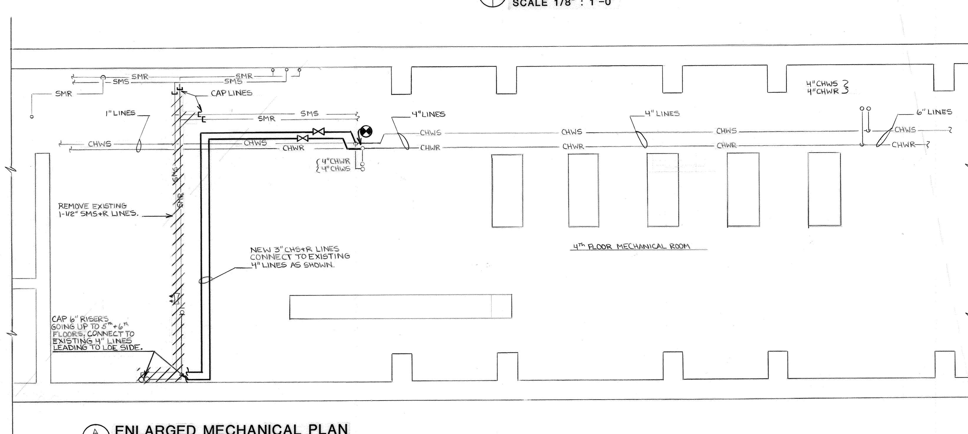
ENLARGED MECHANICAL PLAN SCALE 1/4" : 1'-0"
