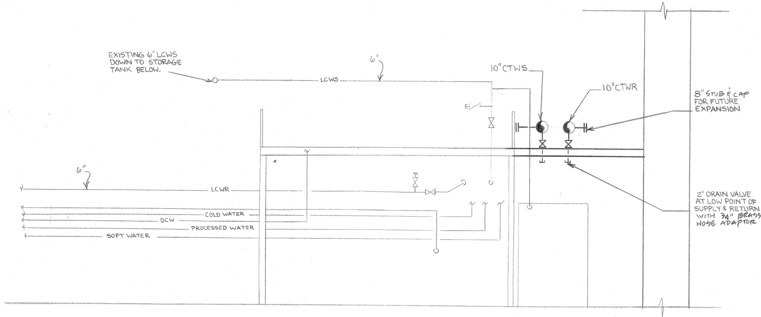
SECTION A SCALE 1/4" : 1'-0"
