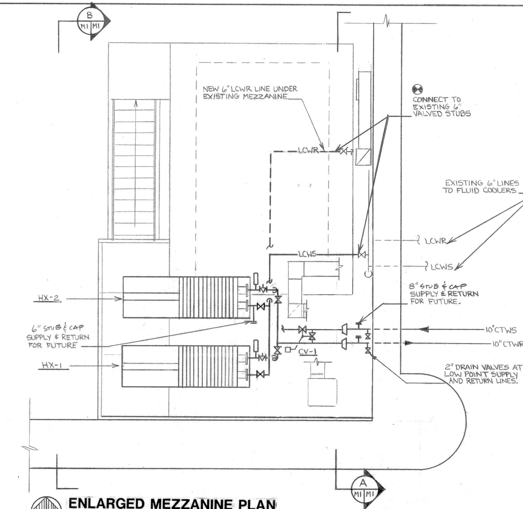
ENLARGED MEZZANINE PLAN SCALE 1/4" : 1'-0"
