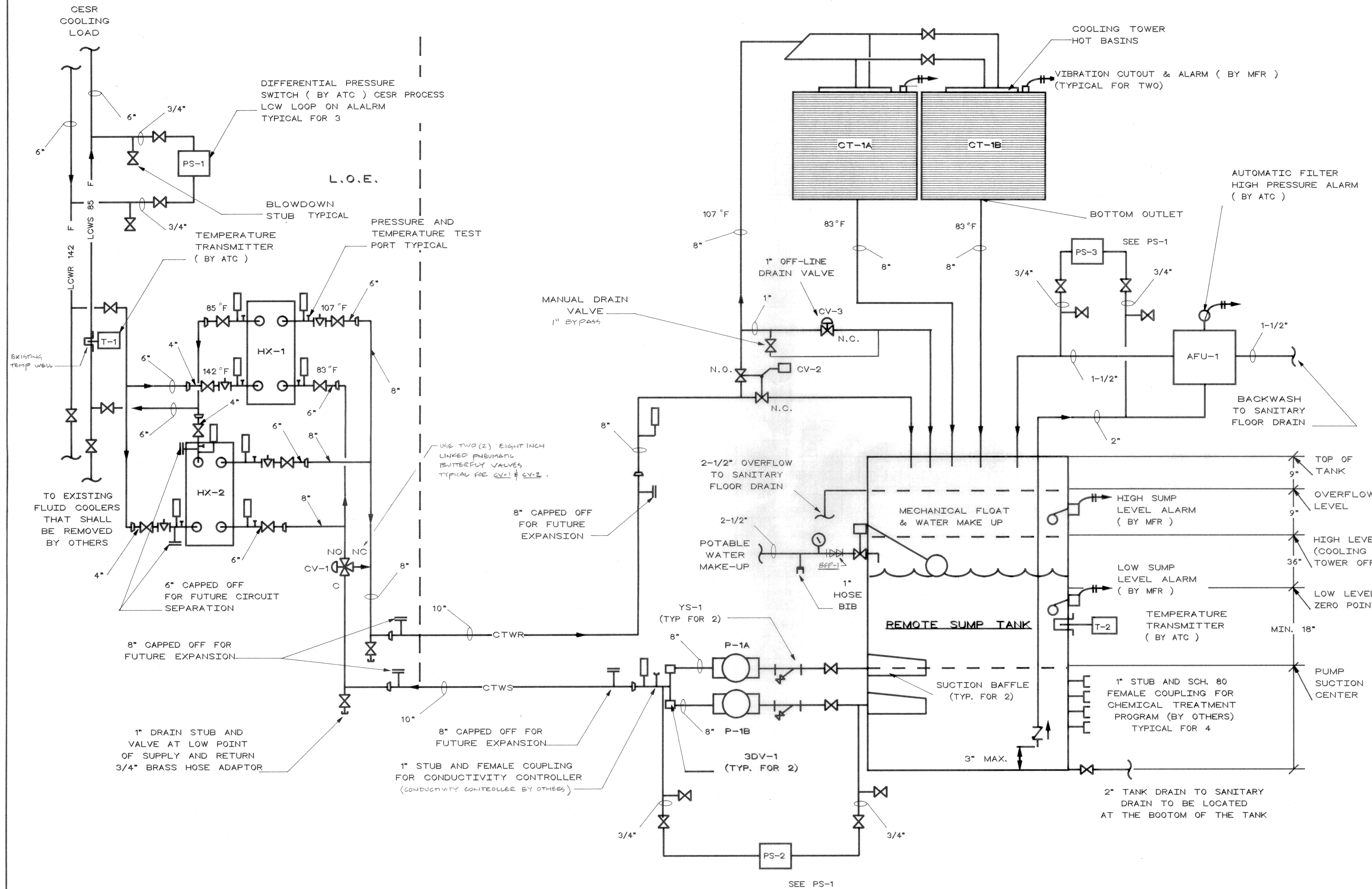
CESR COOLING TOWER FLOW SCHEMATIC NOT TO SCALE
