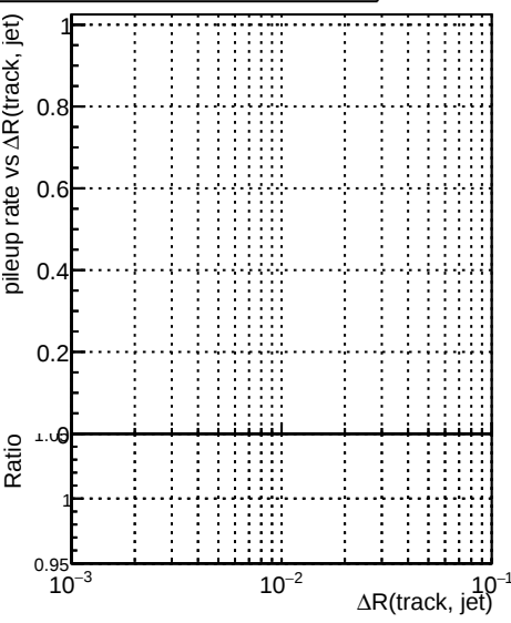
Pileup rate vs \Delta R
