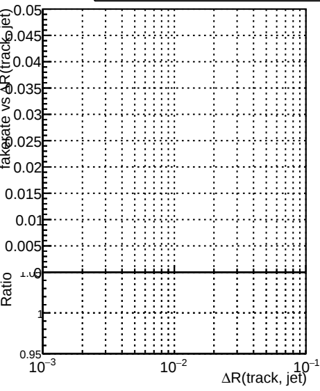
Fake rate vs \Delta R
