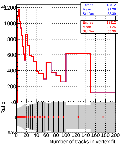
ReconstructedAllAssoc2Gen_NumTracks
