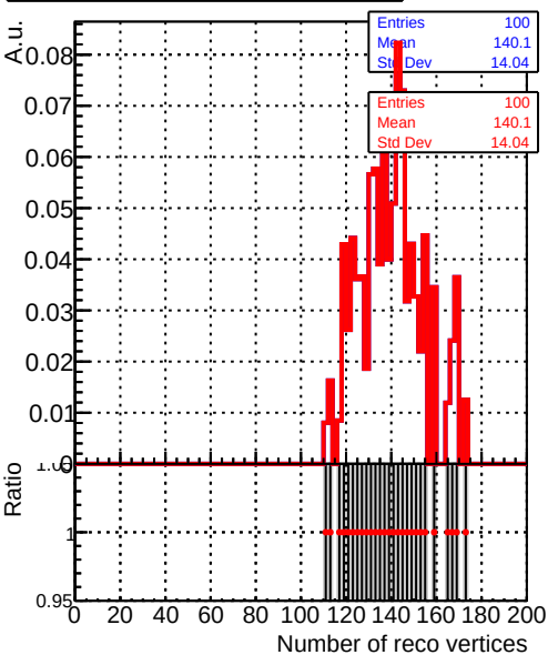
ReconstructedAllAssoc2Gen_NumVertices
