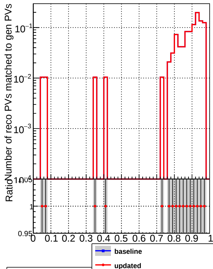
RecoPVAssoc2GenPVmatched_missing
