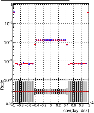
(PacketCandidate::bestTrack() - reco::Track)reco::Track in cov(dx, dsz)
