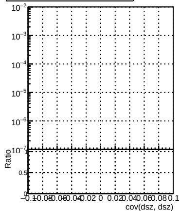
(PacketCandidate::bestTrack() - reco::Track)reco::Track in cov(dsz, dsz) with over- and underflow, and sign flip
