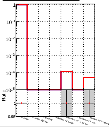
(PacketCandidate::bestTrack() - reco::Track)reco::Track in cov(dx, dxy) status
