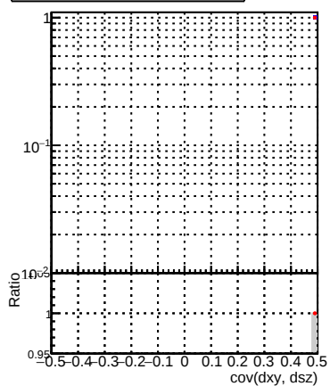
(PacketCandidate::bestTrack() - reco::Track)reco::Track in cov(dx, dsz) with over- and underflow, and sign flip
