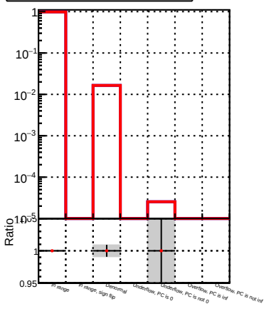
(PacketCandidate::bestTrack() - reco::Track)reco::Track in cov(dx, dsz) status
