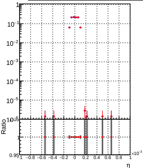
baseline updated
