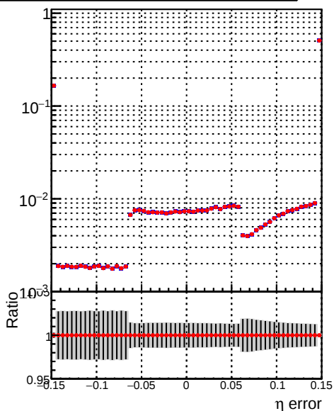
baseline updated
