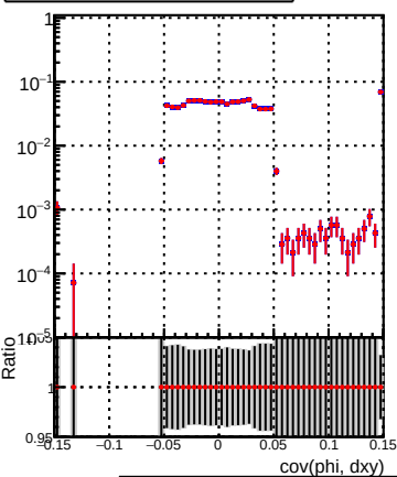
(PacketCandidate::bestTrack() - reco::Track)(reco::Track in cov(phi, dxy) status)
