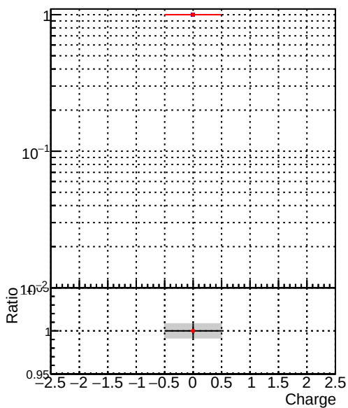
PackedCandidate::bestTrack() - reco::Track in charge() Legend: baseline (blue line with circles), updated (red line with circles)
