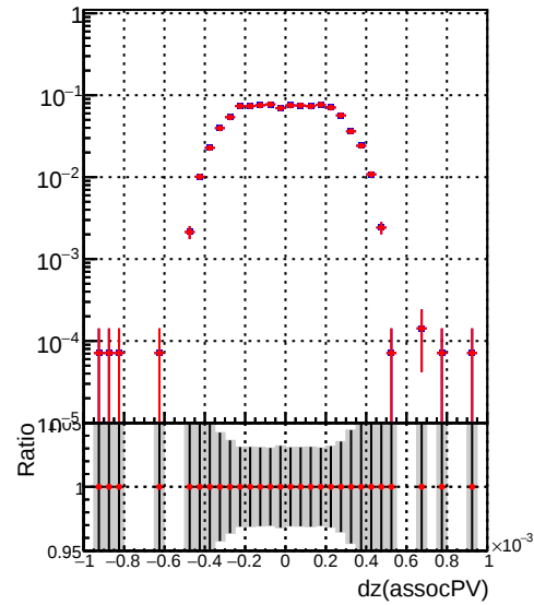
(PackedCandidate::dz(assocPV) - reco::Track::dz(assocPV))/reco::Track
