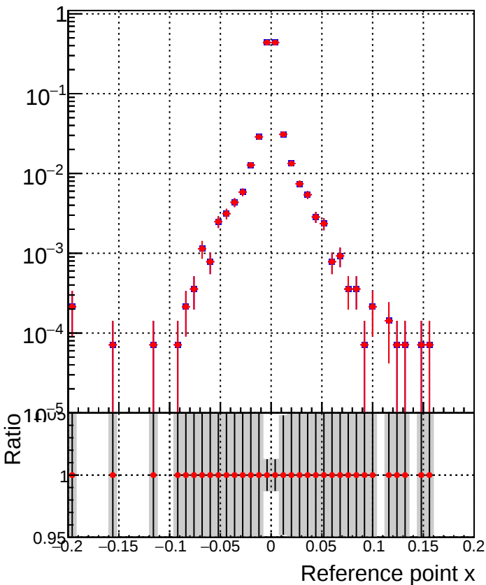
PackedCandidate::bestTrack
