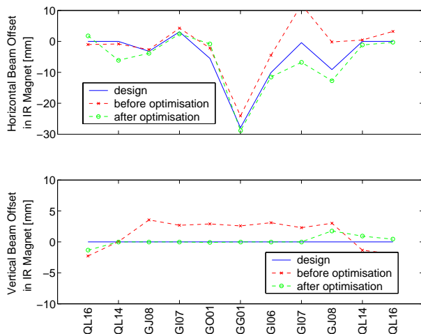
Figure 3: BBA measurements of beam positions before and after orbit optimization across the interaction region with the experiment ZEUS.
